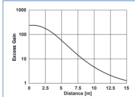
EXCESS GAIN
